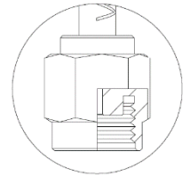
DETAIL C SCALE 2 : 1
