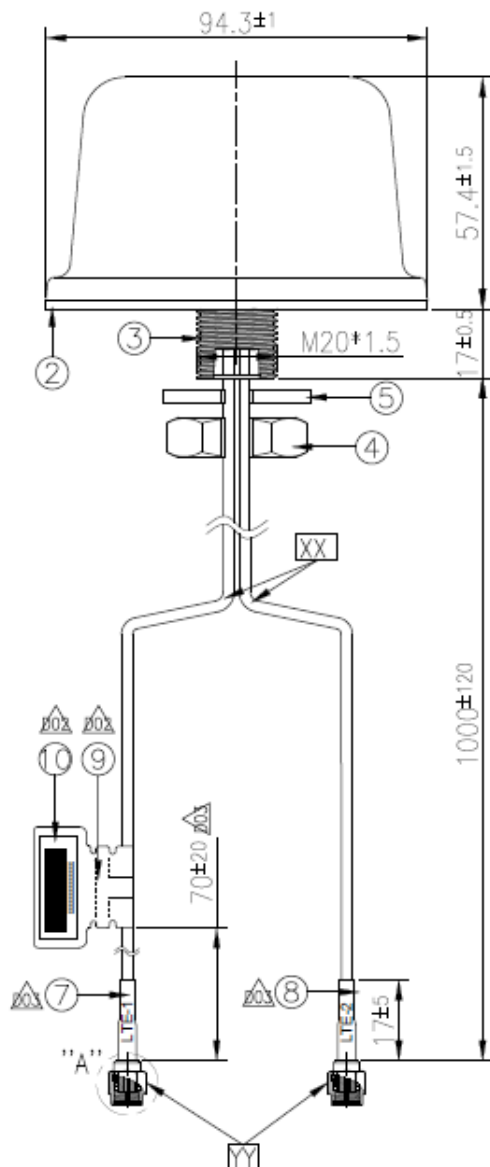
Front View
